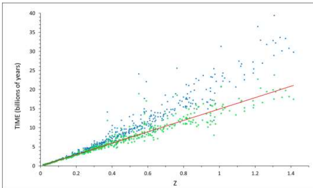
Fig. 1 The redshift of type 1A supernovae with uncorrected and corrected time since emission.
