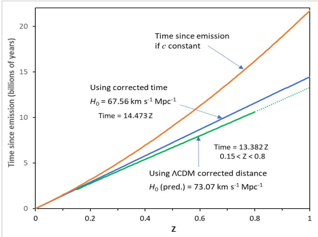
Fig. 5. Comparison of the effect of the correction factors on fit to DES data.
